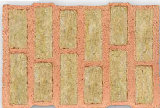
Porotherm 38 W.i Plan
